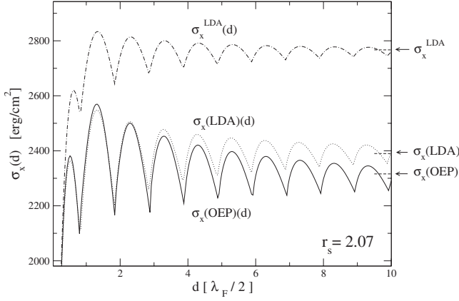
FIG. 5. Exchange surface energy, as a function of slab width d , for r_s=2.07 , from Eq. (43), with l=x . Full line, OEP results; dotted line, LDA results; dash-dotted line, standard LDA-exchange results. The three arrows on the right denote the extrapolated asymptotic values \sigma_x(\text{OEP}) \rightarrow 2316 erg/cm 2 , \sigma_x(\text{LDA}) \rightarrow 2390 erg/cm 2 , and \sigma_x^{\text{LDA}} \rightarrow 2767 erg/cm 2 .
