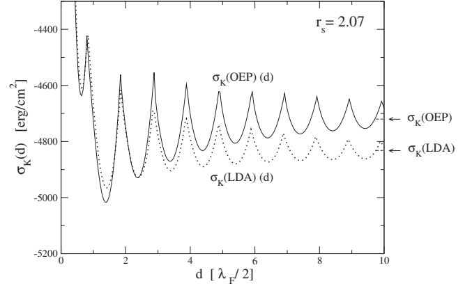
FIG. 3. Kinetic surface energy, as a function of slab width d , for r_s=2.07 , from Eq. (43), with l=K . Full line, OEP results; dotted line, LDA results. The two arrows on the right denote the extrapolated asymptotic values \sigma_K(\text{OEP}) \rightarrow -4720 \text{ erg/cm}^2 , \sigma_K(\text{LDA}) \rightarrow -4832 \text{ erg/cm}^2 .
