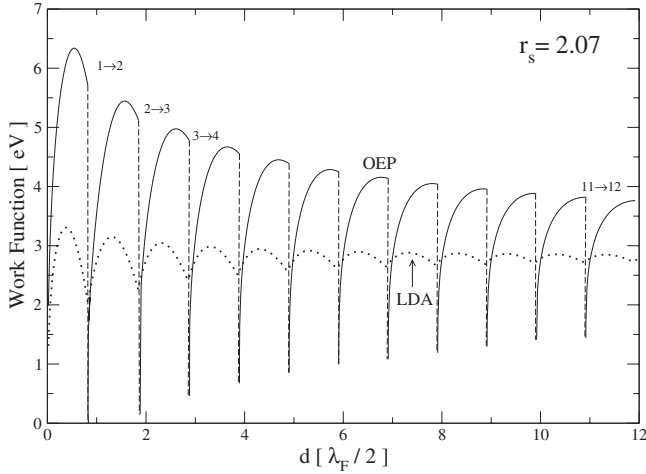
FIG. 6. Slab work function versus slab width d for r_s=2.07 . Full line, OEP result; dotted line, LDA result. Occupation events corresponding to transitions from a slab with m occupied SDL toward m+1 occupied SDL are denoted as m \rightarrow m+1 .
