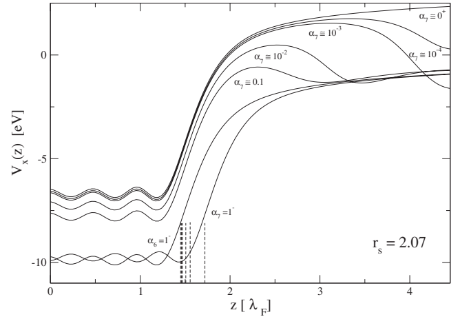
FIG. 7. Self-consistent OEP exchange potential, around the 6 \rightarrow 7 SDL transition, for r_s=2.07 . The origin of coordinate z for each slab has been taken at the slab center. The position of the right slab edge has been indicated by a vertical dashed line for each case.
