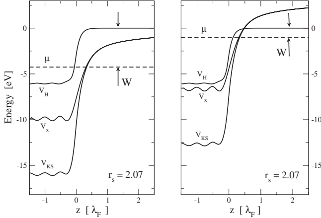
FIG. 8. Left: electronic structure of the slab for \alpha_6=1^- . Right: electronic structure of the slab for \alpha_7=0^+ . The work-function W jumps discontinuously from its left large value toward the smaller right value. Slab edge is at z=0 .
