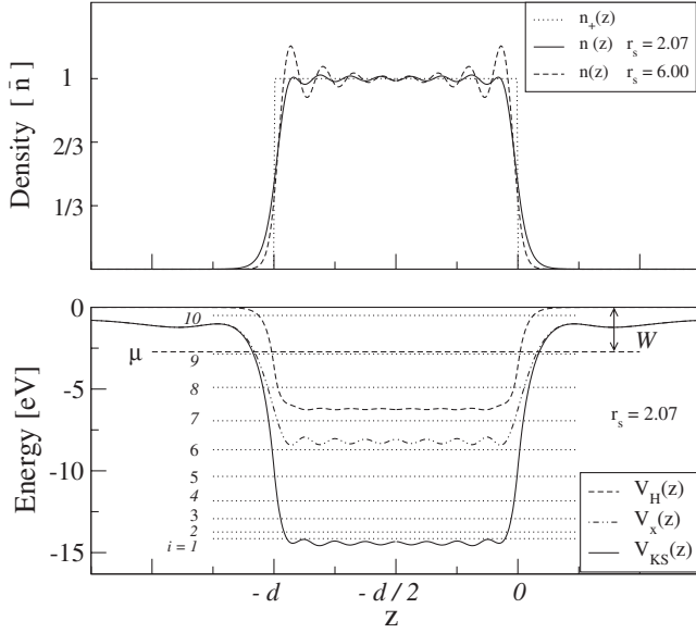
FIG. 1. Main features of the jellium-slab model of metal surfaces. Top panel: normalized jellium density [n_+(z)] and the self-consistent OEP electron density n(z) for two different values of the electron-density parameter r_s . Lower panel: OEP Hartree, exchange, and Kohn-Sham potentials for r_s=2.07 . Dotted lines denote KS eigenvalues, \epsilon_F is the Fermi energy, and W is the work function. d=4\lambda_F .
