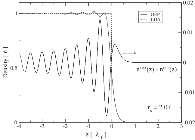
FIG. 2. LDA and OEP self-consistent electron densities and their difference for d=8\lambda_F and r_s=2.07 . Note that n^{\text{LDA}}(z) is slightly more diffuse than n^{\text{OEP}}(z) , as n^{\text{LDA}}(z) - n^{\text{OEP}}(z) > 0 for z outside the jellium edge (in the vacuum).
