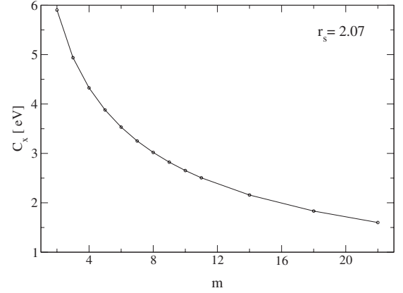
FIG. 9. Exchange-driven discontinuity C_x(m) for increasing number of occupied slab levels, as follows from Eq. (51).
