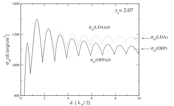
FIG. 4. Electrostatic surface energy, as a function of slab width d , for r_s=2.07 , from Eq. (43), with l=\text{el} . Full line, OEP results; dotted line, LDA results. The two arrows on the right denote the extrapolated asymptotic values \sigma_{\text{el}}(\text{OEP}) \rightarrow 1103 \text{ erg/cm}^2 , \sigma_{\text{el}}(\text{LDA}) \rightarrow 1172 \text{ erg/cm}^2 .
