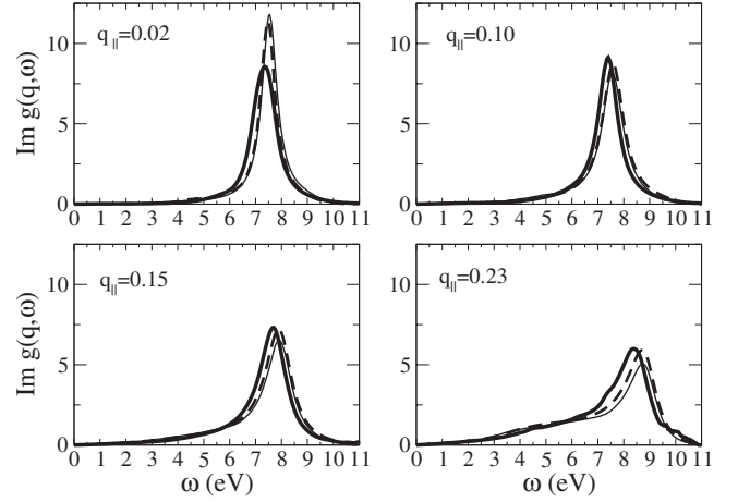
FIG. 1. Imaginary part of the RPA surface-response function of Mg(0001) \text{Im } g(\mathbf{q}, \omega) , as a function of \omega , for various values of the magnitude q of the wave vector. The thick solid line represents self-consistent first-principles calculations, the dashed line represents the corresponding results obtained for a semi-infinite jellium surface, and the thin solid line represents the corresponding results obtained by using the 1D model potential of Ref. 22.
