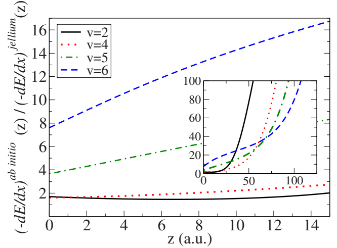
FIG. 3. (Color online) Ratio (-dE/dx)^{ab\ initio}(z)/(-dE/dx)^{jellium}(z) versus z for a recoilless particle of charge Z_1=1 moving with various velocities outside the Mg(0001) surface. In the inset, larger distances z from the surface are considered.
