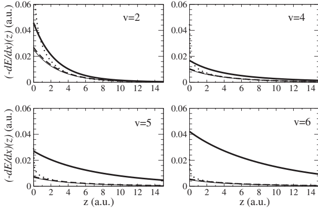
FIG. 2. Stopping power of Mg(0001) versus z for a recoilless particle of charge Z_1=1 moving with various velocities. The thick solid line represents self-consistent first-principles calculations. The dashed and thin solid lines represent the corresponding results obtained for a semi-infinite jellium surface and by using the 1D model potential of Ref. 22, respectively. The dotted lines represent the classical energy loss of Eq. (24).
