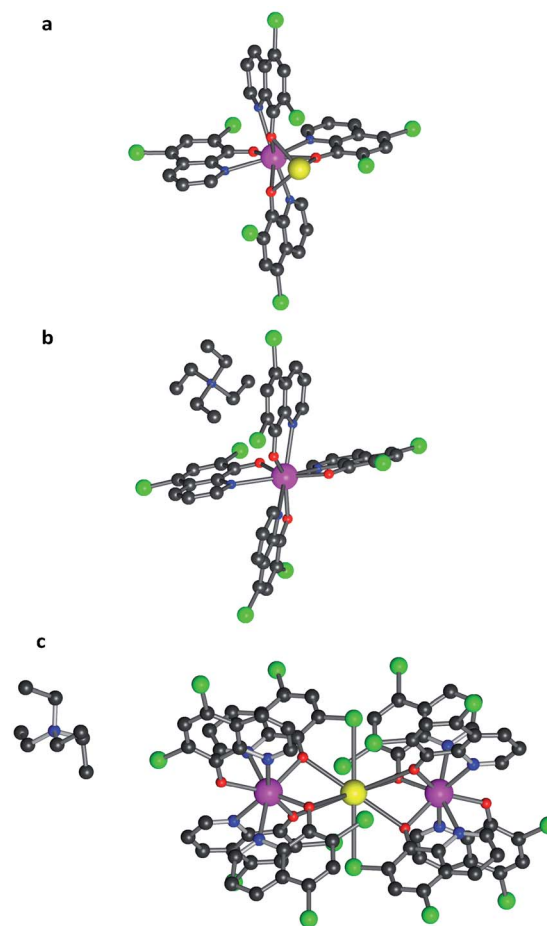
Fig. 1 The molecular structure of the compounds. (a) Na[Ln(5,7Cl 2 q) 4 ] (in short NaLnClq with Ln = Y (1), Tb (2) or Dy (3)); (b) NEt 4 [Dy(5,7Cl 2 q) 4 ] (4); (c) K 0.5 (NEt 4 ) 0.5 [Dy(5,7Cl 2 q) 4 ] (5). The central lanthanoid ion is in pink, oxygen in red, nitrogen in blue, carbon in black, chlorine in green and sodium (in a) and potassium (in c) in yellow. Hydrogen atoms have been omitted for clarity.
